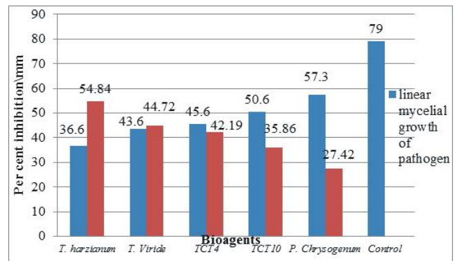
Fig. 1 : In vitro evaluation of fungal antagonists against Alternaria porri .
