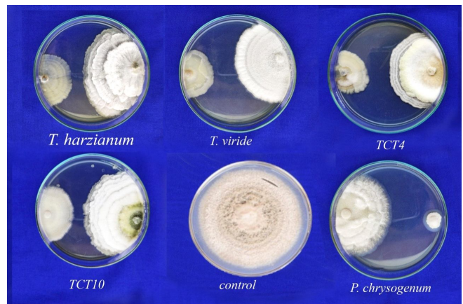
Fig. 2 : In vitro evaluation of fungal antagonists against A. porri .
